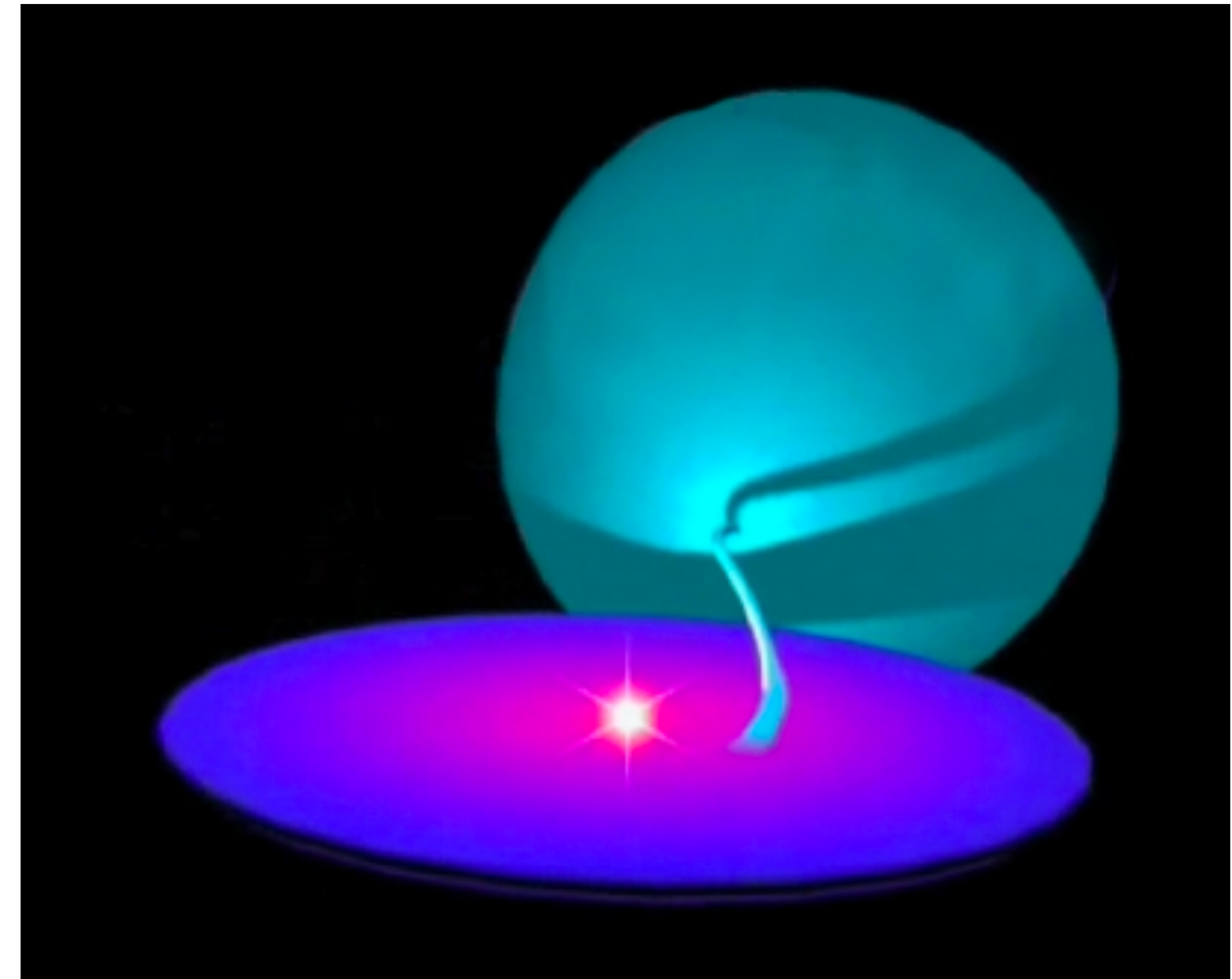
Her X-1
